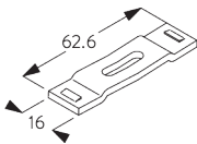
SG 3113 Bracket
