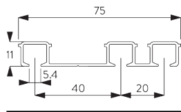
SG 6293p Profile
