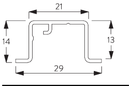
SG 11231 Recess profile
