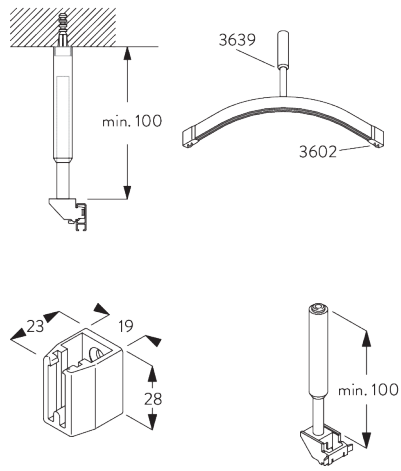
SG 3602 Wall support
