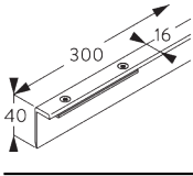
SG 6512 Connection bridge
